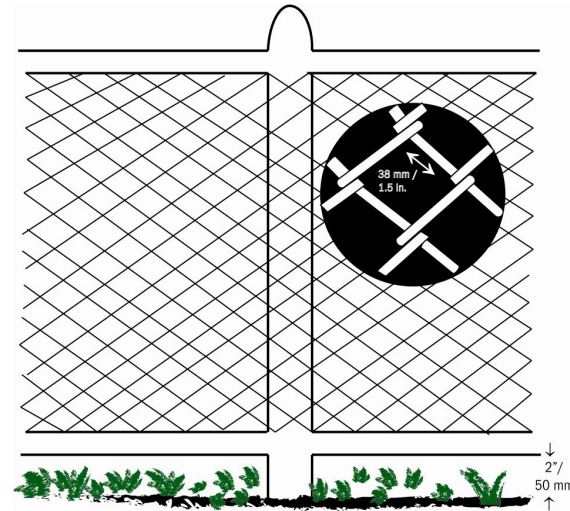
Figure 4: Chain Link Openings
